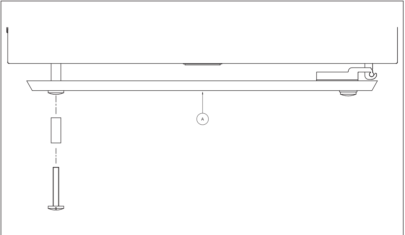
Fig. 7: slide the H26 Nylon spacer on the M6X40 screw provided and fasten it, by passing through the hole in the hole in the glass, to the upper hole in the hood cylinder, tightening it by hand or using a tool or coin.
