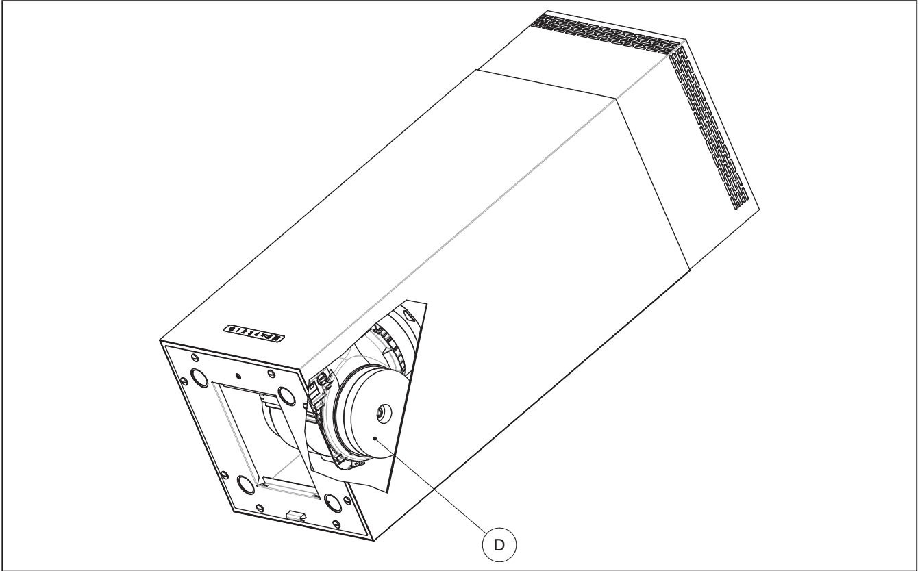
Fig. 8: if a filtering hood is being installed, you must request two carbon filters (D) (supplied as a separate accessory). Proceed to the insertion of the drawer-type carbon filter with the required type of slot system.
