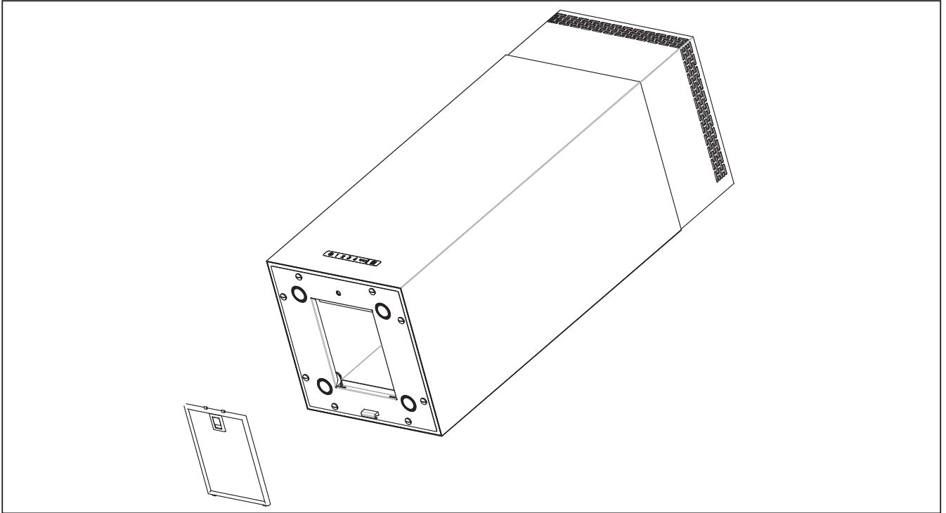
Fig. 4: mount the grease filter on the hood cylinder with the metal handle.
